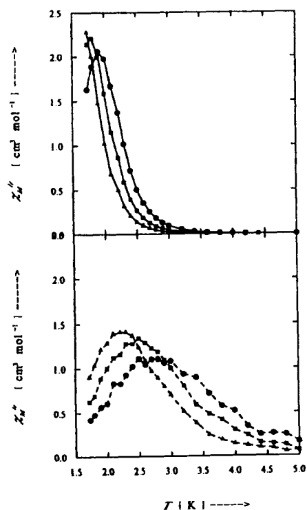
FIGURE 9 Out-of-phase AC magnetic susceptibility for complex 7 as a microcrystalline solid (top) and as a frozen \text{CD}_2\text{Cl}_2/\text{C}_6\text{D}_5\text{CD}_3 glass (bottom).
