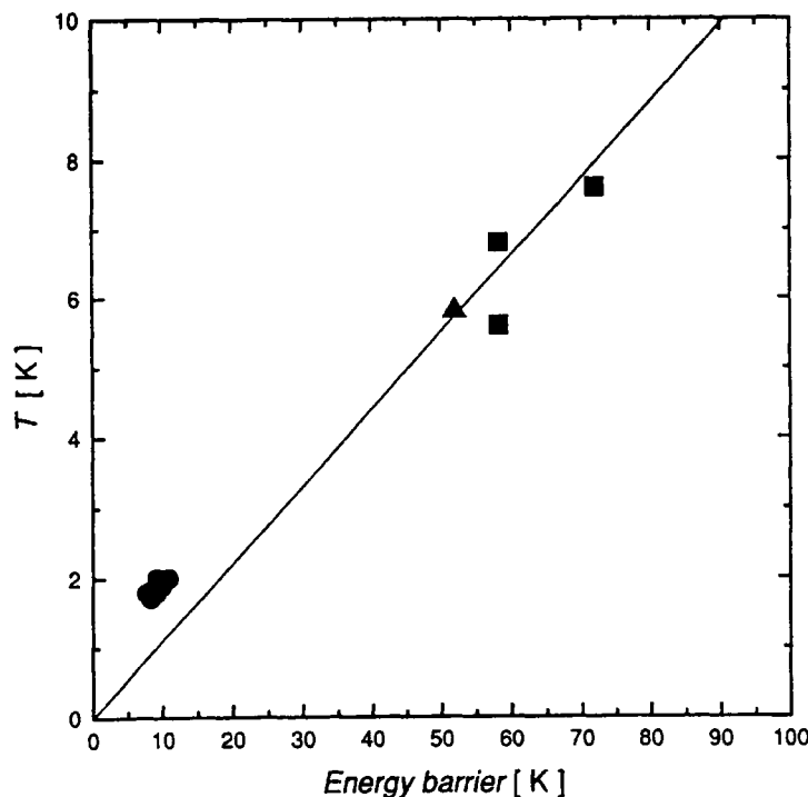
FIGURE 10 Plot of the temperature at which there is a maximum in \chi_m'' at 997 Hz vs the calculated energy barrier for relaxation of magnetization. Data are presented for [\text{Mn}_{12}] (■), [\text{Mn}_{12}]^+ (▲) and [\text{Mn}_4] (●) complexes.
