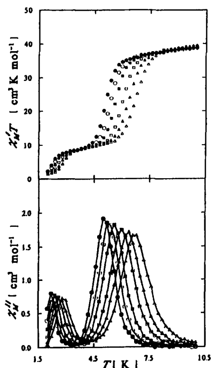
FIGURE 3 AC magnetic susceptibility for complex 2 \cdot \text{H}_2\text{O} . At the top and bottom, respectively, are plotted \chi'_m T vs T and \chi''_m vs T , where \chi'_m and \chi''_m are the in-phase and out-of-phase signals, respectively. Data are at 997 ( \Delta ), 499 ( \blacktriangle ), 250 ( \square ), 100 ( \blacksquare ), 500 ( \circ ) and 25 ( \bullet ) Hz frequencies.
