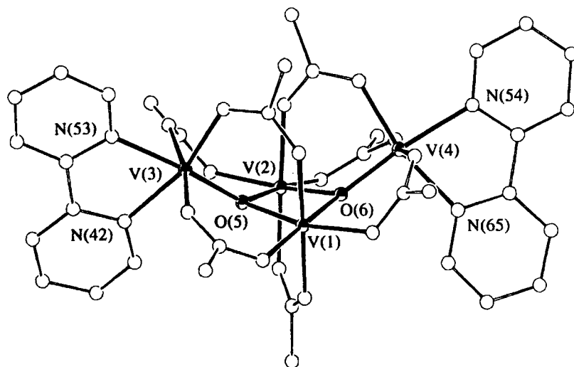
FIGURE 13 The structure of [\text{V}_4\text{O}_2(\text{O}_2\text{Cet})_7(\text{bpy})_2]^+ (10) with Me groups omitted.
