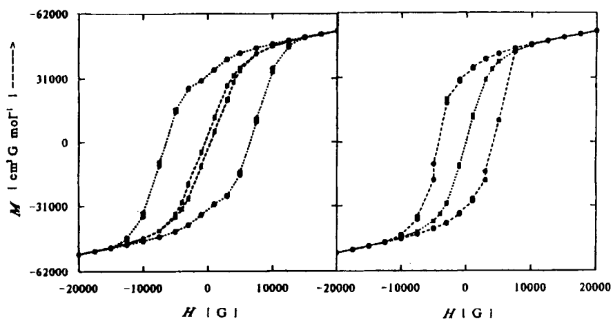
FIGURE 5 Hysteresis loops for 2 \cdot \text{H}_2\text{O} (left) and 4 (right) at 2.2 (●) and 2.8 (■) K.
