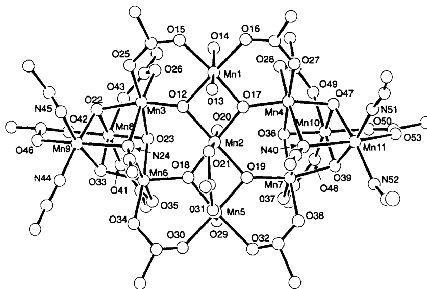
FIGURE 11 The structure of [\text{Mn}_{11}\text{O}_{10}(\text{NCO})_6(\text{O}_2\text{CPh})_{11}(\text{H}_2\text{O})_4]^{2-} ( 9 ); only the ipso C atom of each Ph ring is shown.
