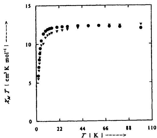
FIGURE 8 DC magnetic susceptibility data in a 10 kG applied field for [\text{Mn}_4\text{O}_3\text{Cl}(\text{O}_2\text{CMe})_3(\text{dbm})_3] (7), plotted as \chi_M T vs T . Data are for a parafilm-restrained microcrystalline solid (●) and a frozen \text{CD}_2\text{Cl}_2/\text{C}_6\text{D}_5\text{CD}_3 glass (▼).
