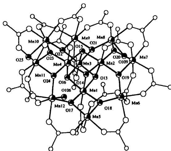
FIGURE 1 The structure of [\text{Mn}_{12}\text{O}_{12}(\text{O}_2\text{Cet})_{16}(\text{H}_2\text{O})_3] (2) with Me groups omitted. The metal atoms in the central cubane are \text{Mn}^{\text{IV}} and the other metal atoms are \text{Mn}^{\text{III}} .
