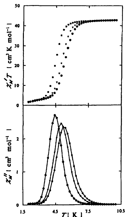
FIGURE 4 AC magnetic susceptibility for complex 4. At the top and bottom, respectively, are plotted \chi'_m T vs T and \chi''_m vs T , where \chi'_m and \chi''_m are the in-phase and out-of-phase signals, respectively. Data are at 499 ( \blacksquare ), 100 ( \blacktriangledown ) and 50 ( \bullet ) Hz frequencies.
