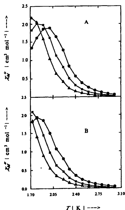
FIGURE 7 Out-of-phase AC magnetic susceptibility for two [\text{Mn}_4\text{O}_3\text{X}]^{6+} complexes with \text{X} = \text{N}_3^- (A) and \text{NCO}^- (B). Data are at 997 (●), 499 (■) and 250 (▲) Hz frequencies.
