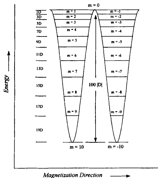
FIGURE 2 Potential energy vs magnetization direction for a complex with S = 10 undergoing axial zero-field splitting (ZFS) with a negative ZFS parameter, D . The energy separation between the M_s = \pm 10 and M_s = 0 levels is |100D| . For S = 19/2 or S = 9 species, related diagrams and energy separations of |90D| and |81D| , respectively, are obtained.
